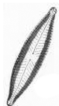
▲ Gambar 4.5 Navicula
